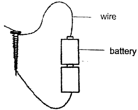
Set-up Q (26 coils)
